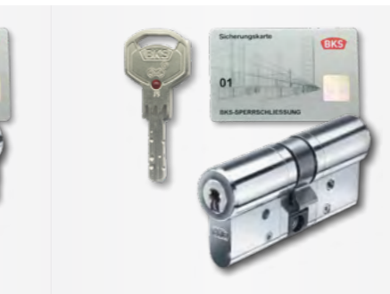
ES 2200 Lock BKS Janus safety profile cylinder with security card according to DIN EN 1303 and DIN 18252
